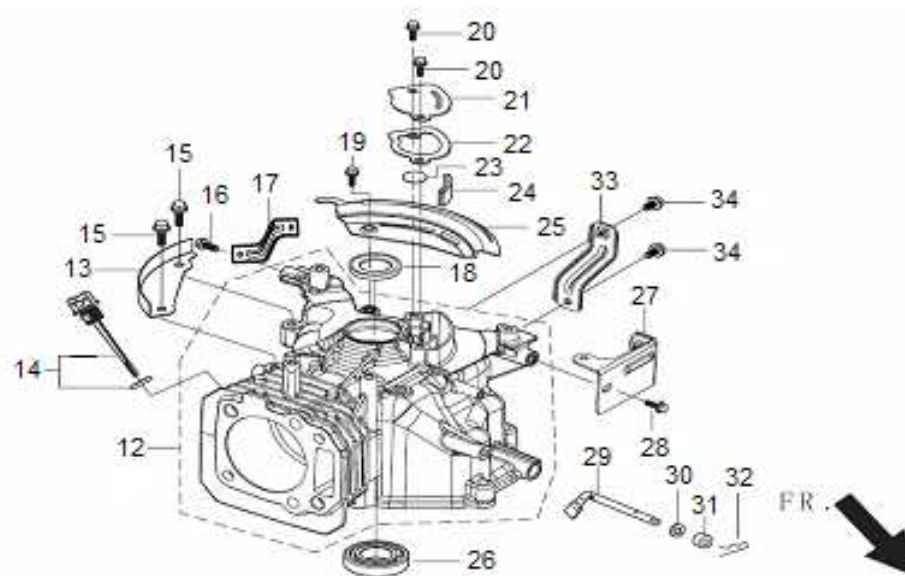
FIG.2 CRANKCASE/GOVERNOR GEAR ASSEMBLY
